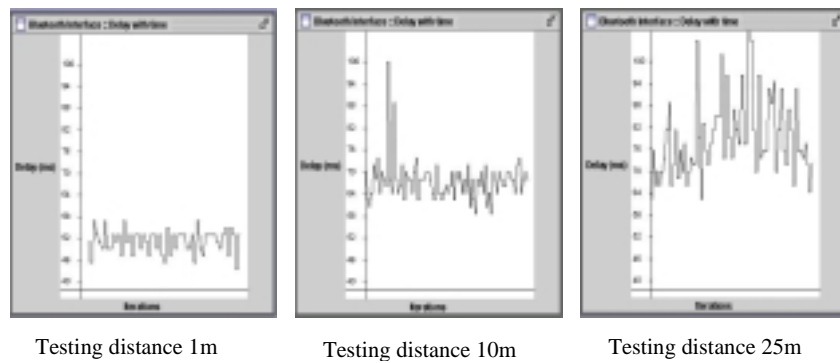
Fig. 10. Delay Performance with distance
