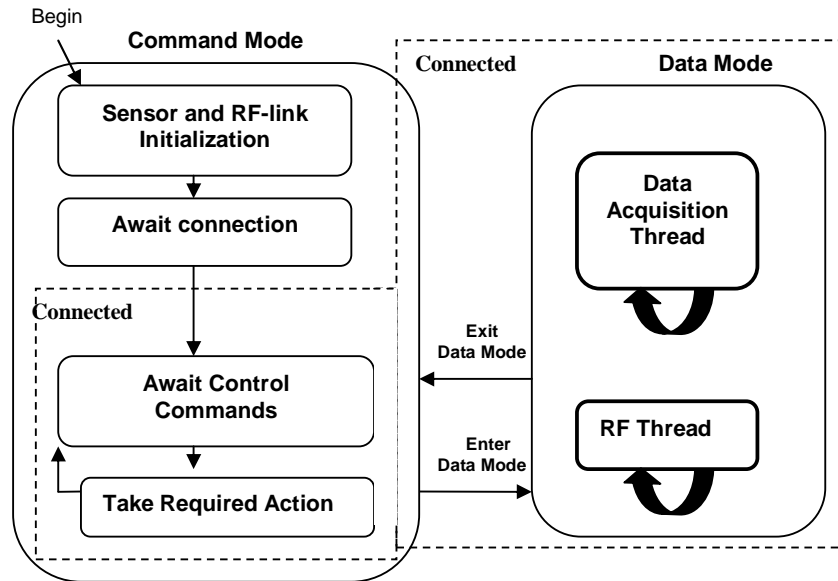
Fig. 5. Software Architecture of the Device (State Machine)
