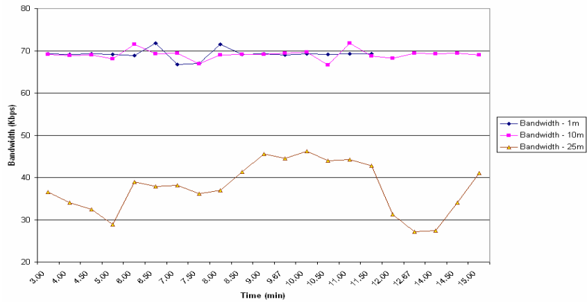
Fig. 11. Bandwidth Performance with distance
