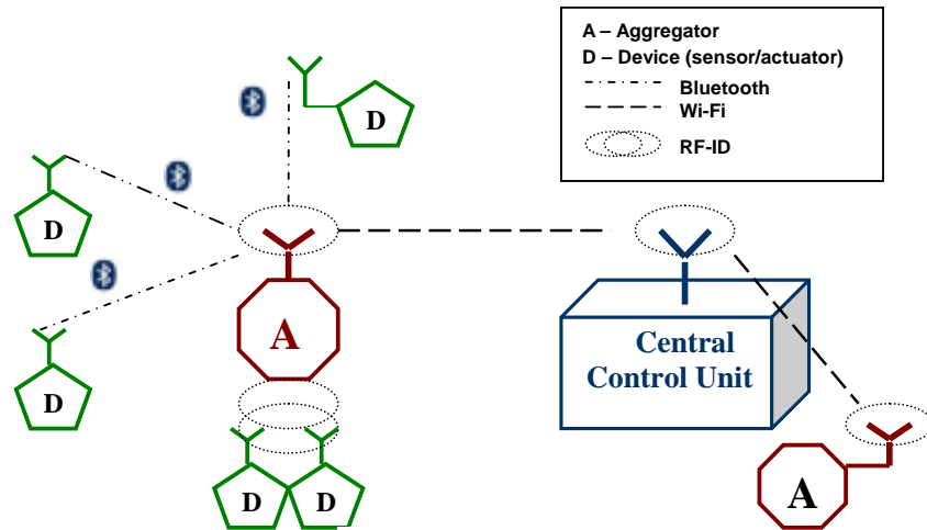
Fig. 2. System Overview
