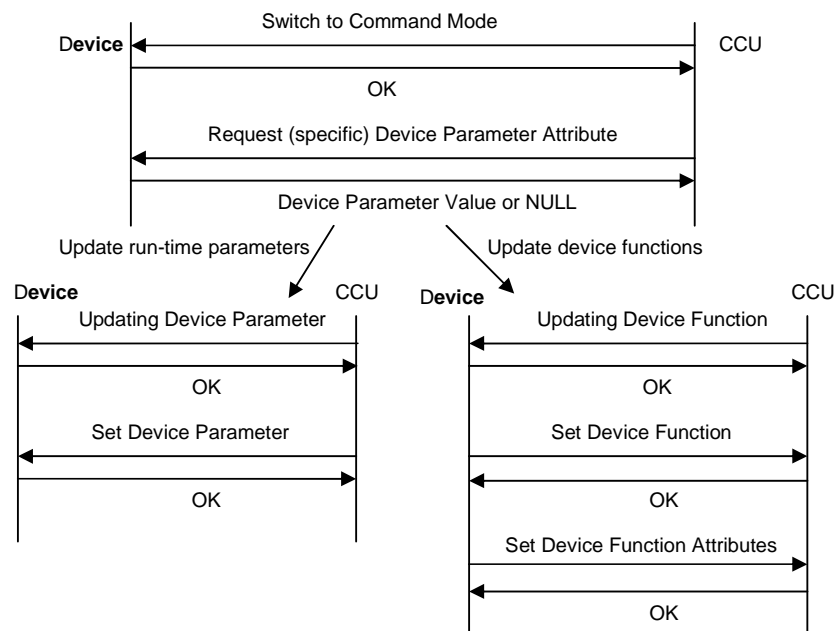
Fig. 7. Message Exchange Flowchart for Device Reconfiguration (OTA)
