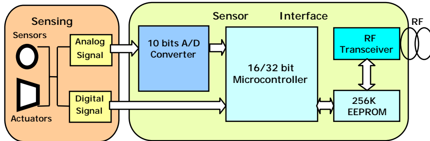
Fig. 4. Hardware design of Intelligent Sensor
